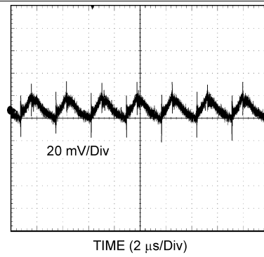
Figure 34. Output Ripple
